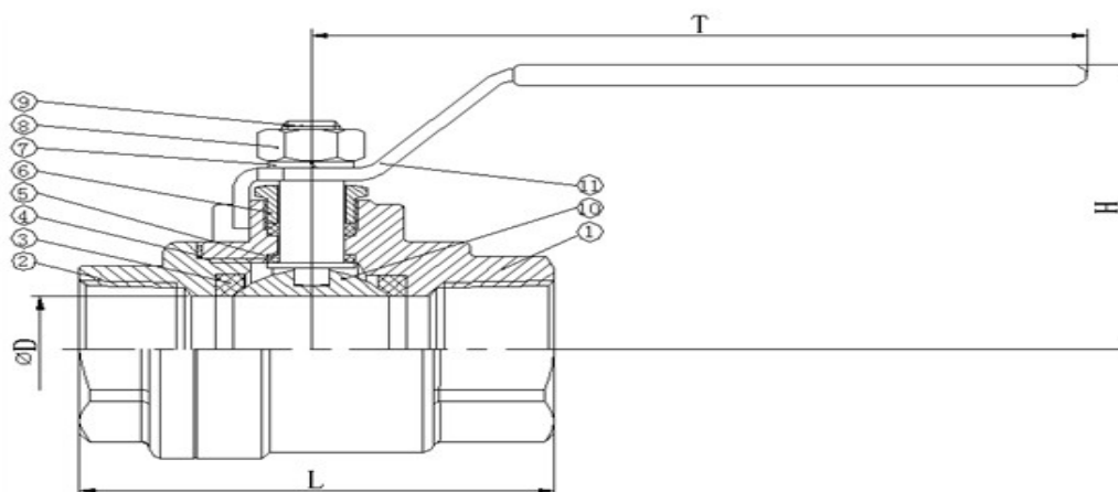
2PC 1000WOG BALL VALVE-SS
